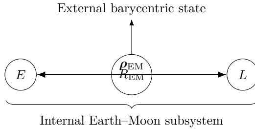
Figure 2: Separation of Earth-Moon external barycentric motion from internal relative motion.
